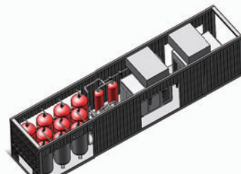
Compressor + tank + dryer +filter system
